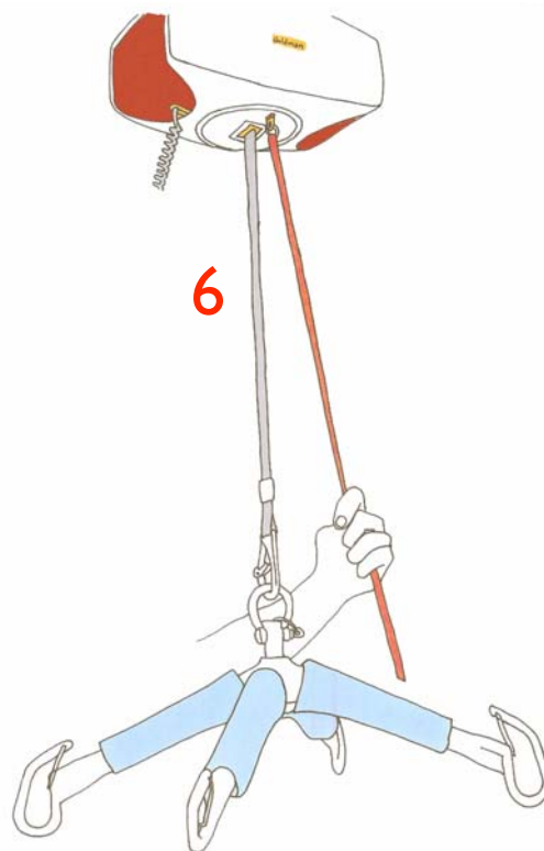
FIG 6. EMERGENCY LOWER- IF THE HOIST FAILS WHILE YOU HAVE A PATIENT IN THE SYSTEM, DETERMINE WHERE TO SAFELY LOWER YOUR PATIENT, THEN PULL AND CONTINUE TO PULL THE RED CORD, THE SYSTEM WILL SLOWLY LOWER THE PATIENT. RELEASING THE PULL ON THE CORD AT ANY TIME STOPS THE PROCESS.
