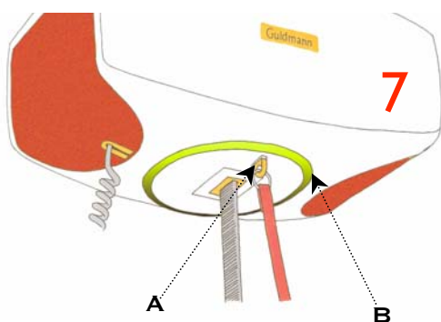
FIG 7. IF THE RED CORD HAS BEEN PULLED, YOU MUST RESET THE HOIST. PUSH YELLOW TAB (A) UNTIL YOU HEAR A CLICK. TO TURN HOIST ON, PRESS HANDSET TOGGLE SWITCH UNTIL GREEN GLOW LIGHT (B) COMES ON.
